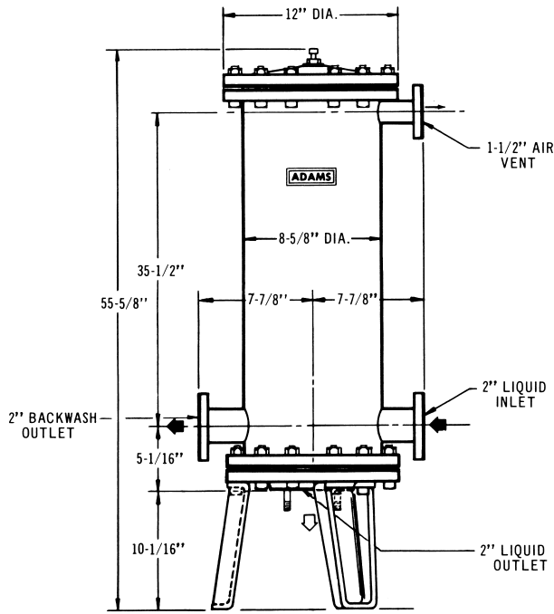
150 Lb. A.S.A. Drilled Flanges. Dimensions vary slightly due to tolerances required for lining.
